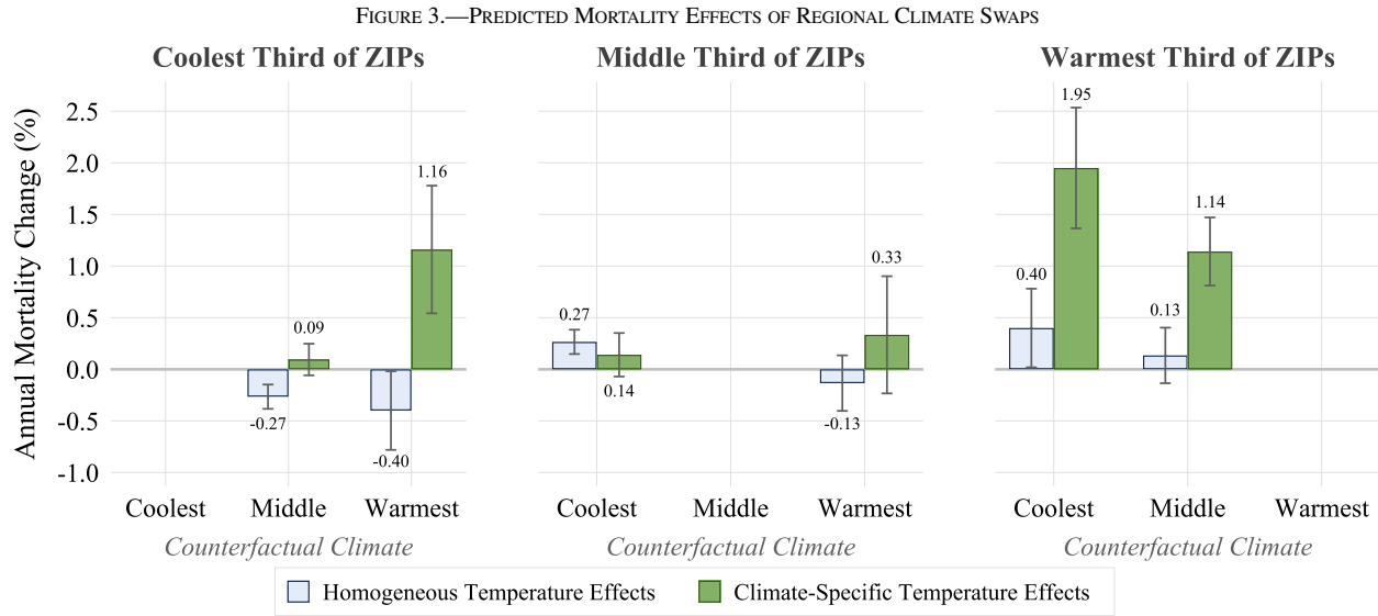
This figure summarizes mortality impacts from counterfactual scenarios in which each of these climate regions' current temperature distribution is replaced by the current distribution of one of the other two climate regions, shown in figure 1.
