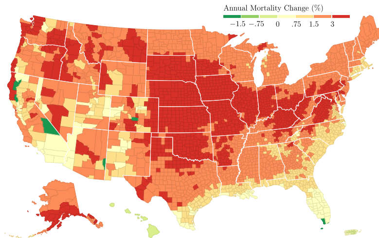
(b) Current Climate Heterogeneity, No Future Adaptation
