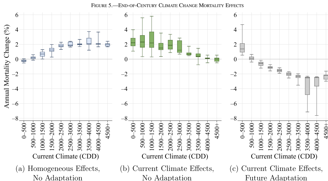
The figure summarizes annual mortality effects of end-of-century (2080–2099) climate change as projected by the meta-model, an average of the 21 NEX-GDDP climate models, under the RCP 8.5 emissions scenario. Effects are calculated for each ZIP code based on the ZIP code's current and future (projected) climates. Panel A reports climate effects under the assumption of homogeneous temperature effects. Panel B reports climate effects that allow for heterogeneous temperature effects based on current climate but do not allow for future adaptation. Panel C reports climate effects that incorporate both current heterogeneity and future adaptation. Box and whisker plots summarize the distribution of climate change effects across ZIP codes in each climate range. Boxes stretch from the 25th percentile (lower hinge) to the 75th percentile (upper hinge). The median is plotted as a line across the box. Whiskers stretch from the 5th percentile to the 95th percentile.
